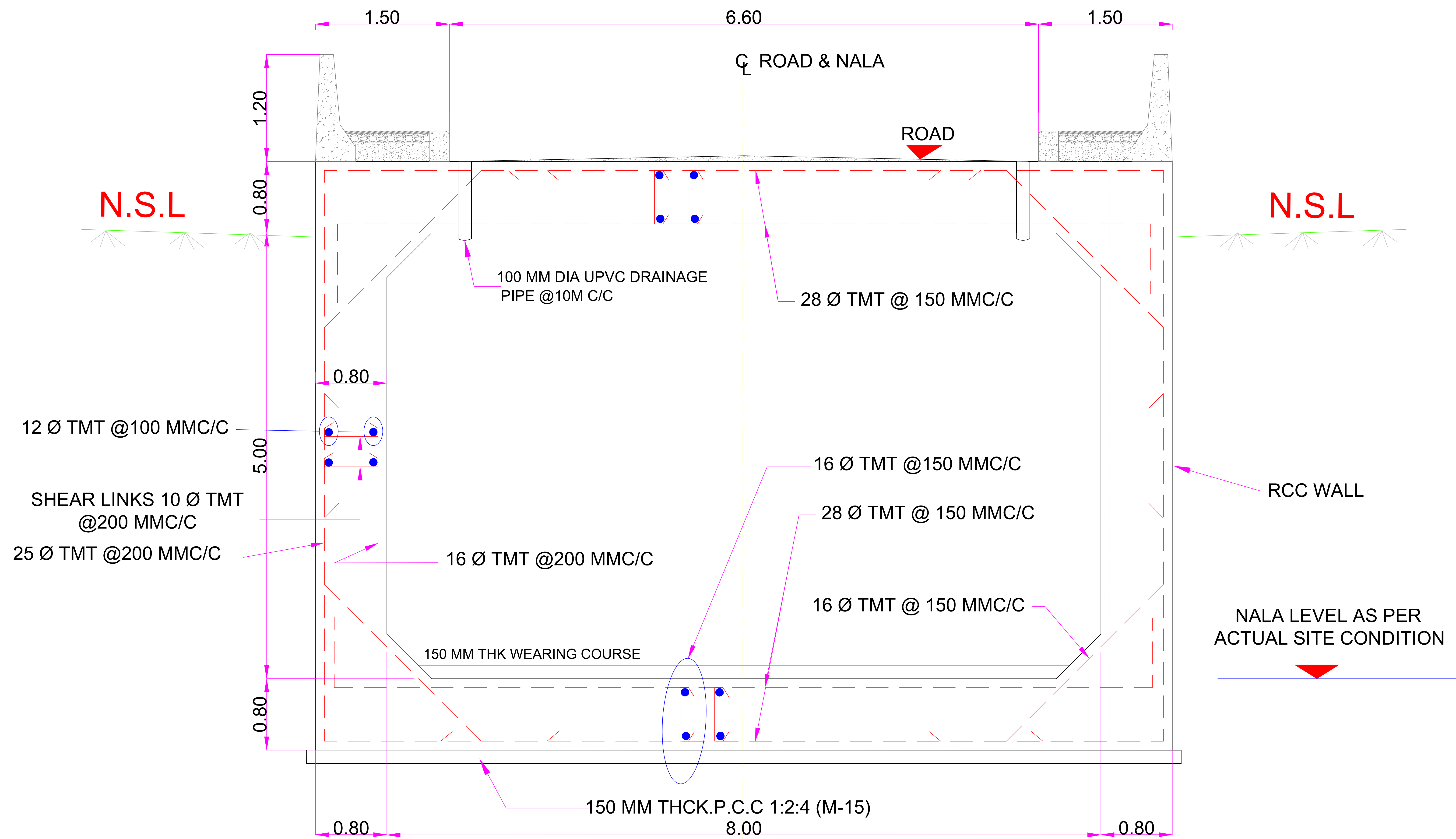
TYPICAL CROSS SECTION OF ROAD & NALA
