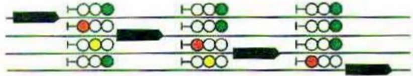
Automatic change of sequence of aspects behind the train in four aspect signalling territory
